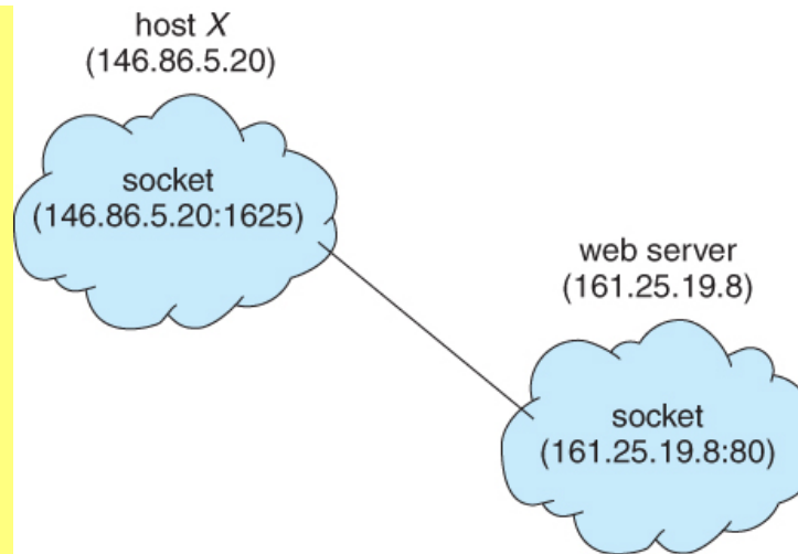
Figure 3.20 - Communication using sockets
