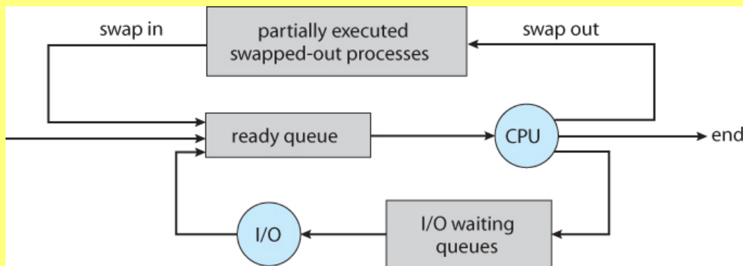
Figure 3.7 - Addition of a medium-term scheduling to the queuing diagram
