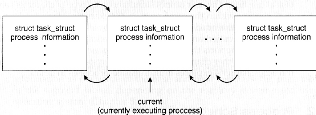
Figure 3.5 Active processes in Linux.
