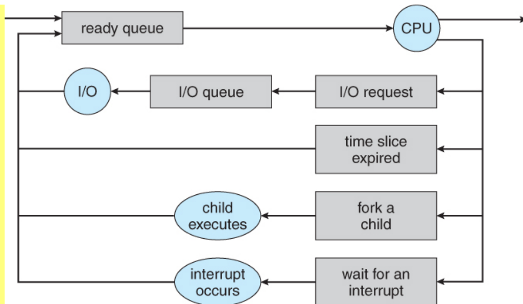
Figure 3.6 - Queuing-diagram representation of process scheduling
