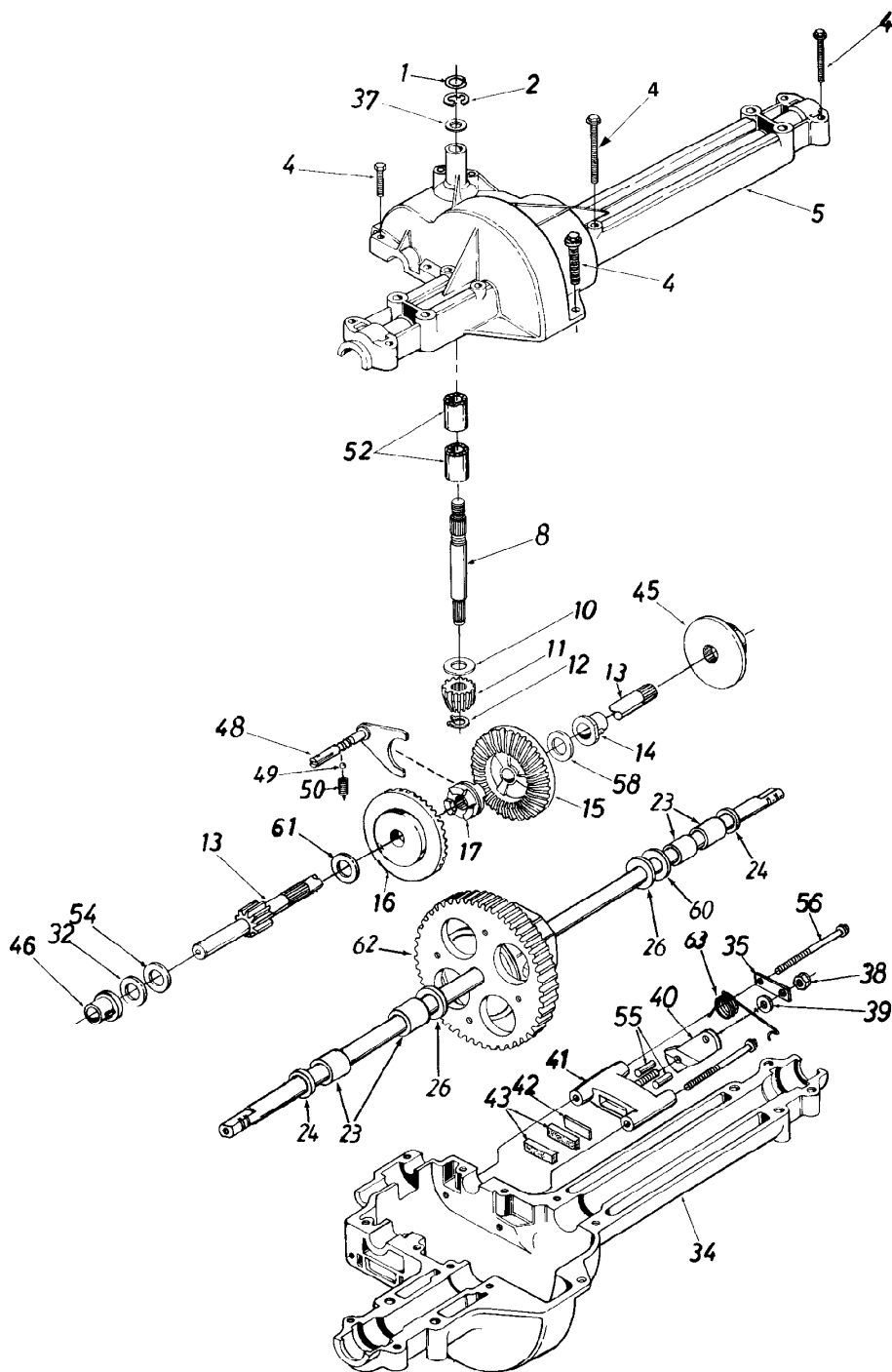
Single Speed Transaxle-RH 618-0163B
